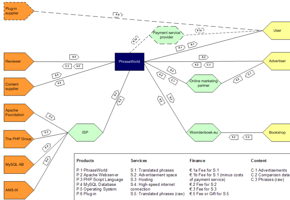
Figure 4: SSN PhraseWorld
