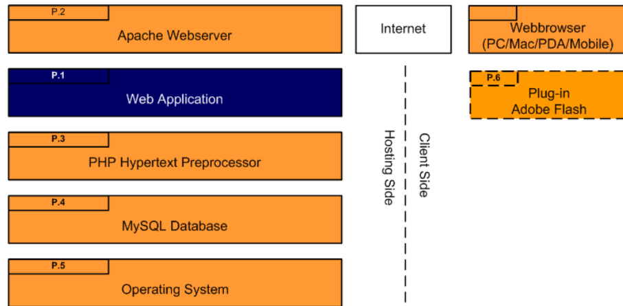
Figure 3: PCD PhraseWorld
